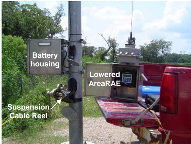
Figure 4. Lowered AreaRAE showing the flagpole-type cable reel.
