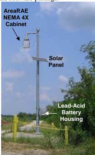
Figure 1. Overview of fenceline monitoring post.
